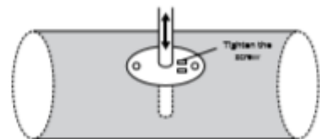
Figure 1b - Mounting the probe in a flange
