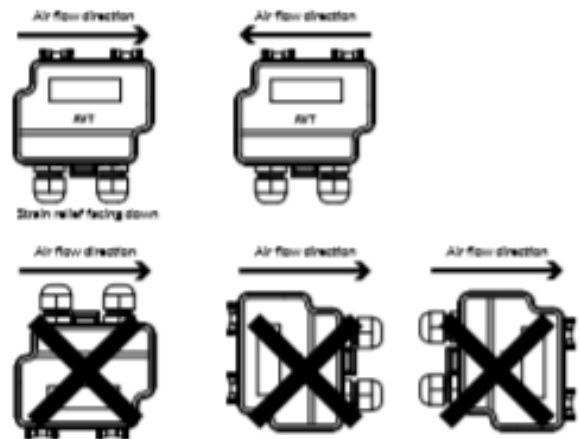
Figure 1c - Mounting orientation
